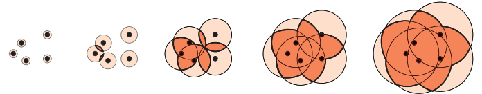
Figure 1: The \alpha -offsets overlaid with the (2, \alpha) -offsets for growing values of \alpha .
