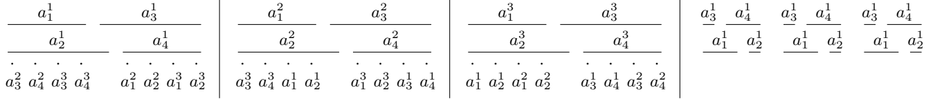
Figure 1: A clique of 12 4-union-intervals satisfying the conditions of Lemma 5 with q = 2
