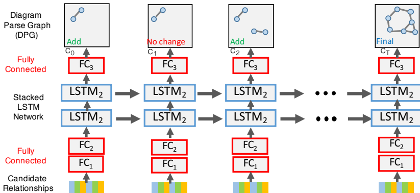
Fig. 2. An overview of the DSDP-NET solution to inferring DPGs from diagrams. The LSTM based network exploits global constraints such as overlap, coverage, and layout to select a subset of relations amongst thousands of candidates to construct a DPG.
