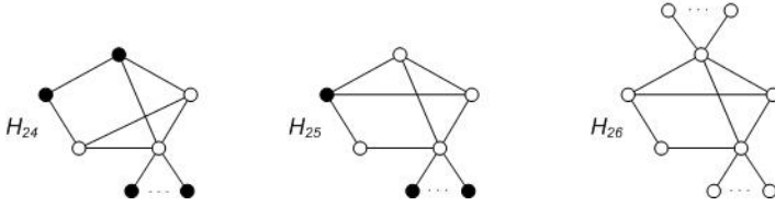
Figure 11: H_{24} \cong G_9 satisfies (1) and H_{25}, H_{26} do not.
