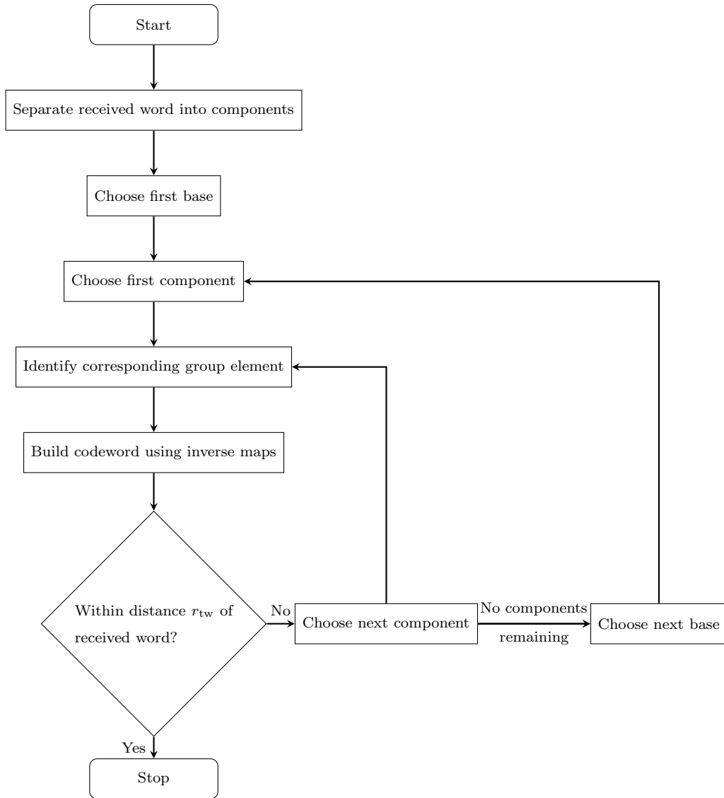
Figure 1: Decoding algorithm for a twisted permutation code
