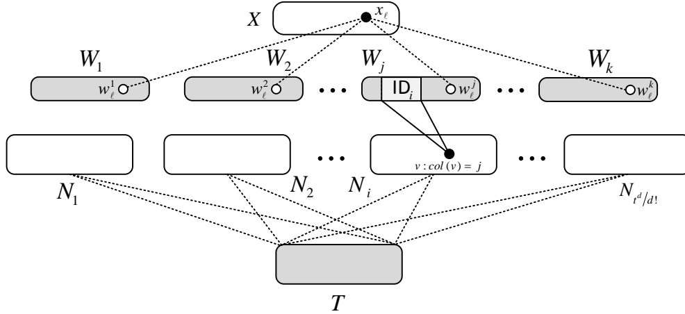
Figure 1: A graphical description of the construction in the first step. The white boxes represent components of terminal vertices, the grey boxes represent components of non-terminal vertices.
