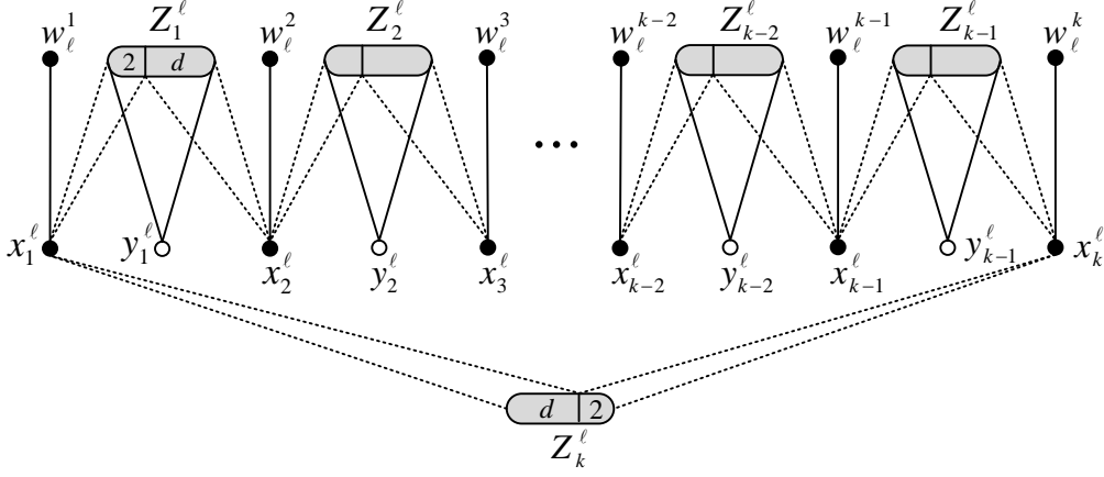
Figure 2: A graphical description of the main part of the equality gadget used to replace x_\ell .
