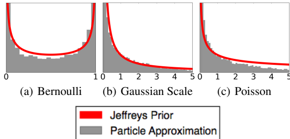
Figure 2: Approximation via Particle Descent.
