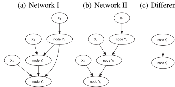
Figure 1: An Illustrative Example of Differential Network Between Two Directed Networks. The error term for each node is not shown for simplicity.
