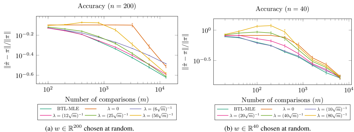
Figure 11: Decaying \lambda with a factor of m^{-1/2} .
