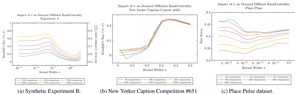
Figure 12: Impact of kernel width on Diffusion RankCentrality for various datasets.
