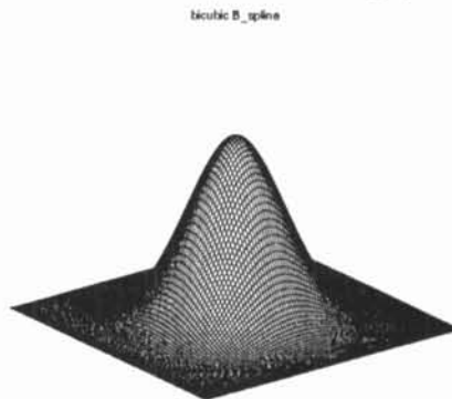
Figure 2: The non-zero portion of a single uniform bicubic B-spline B_{0,0}(x, y) , formed by, uniform cubic B-splines B_0(x), B_0(y) .
