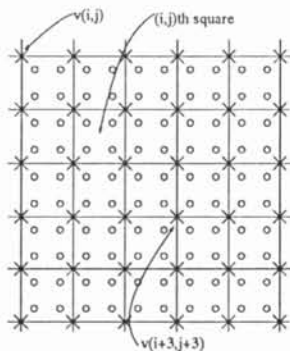
Figure 1: Control vertices, Image pixels for the (i, j) Square Patch.
