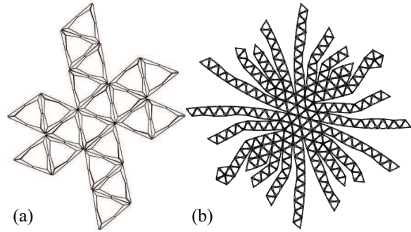
Figure 4: Edge unfoldings of the banded geodomes in Fig. 3.
