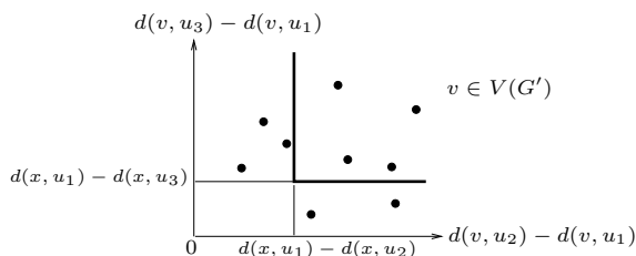
Figure 2: The set of vertices in V(G') to which the shortest path from x goes through u_1 .
