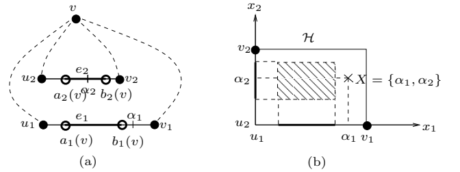
Figure 1: Mapping a 2-center local feasibility test to a 2-dimensional KMP.
