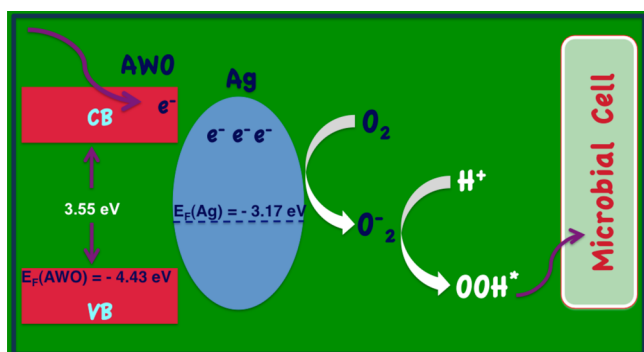
Figure 8. Proposed antimicrobial activity mechanism based on the energy band structure and electron–hole pair transfer and separation in \alpha\text{-Ag}_2\text{WO}_4 with metallic Ag.
