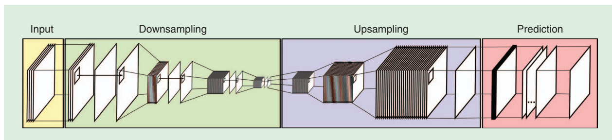
FIGURE 11. The deconvolution network proposed in [92]. The yellow and green parts correspond to a fully convolutional network with a 9 \times 9 -pixels bottleneck; then, a deconvolutional block (purple) leads to predictions of the same size as the input image (in [92], 65 \times 65 pixels).
