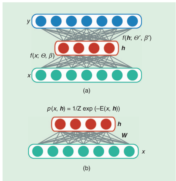
FIGURE 1. A schematic comparison of (a) an AE and (b) an RBM.
