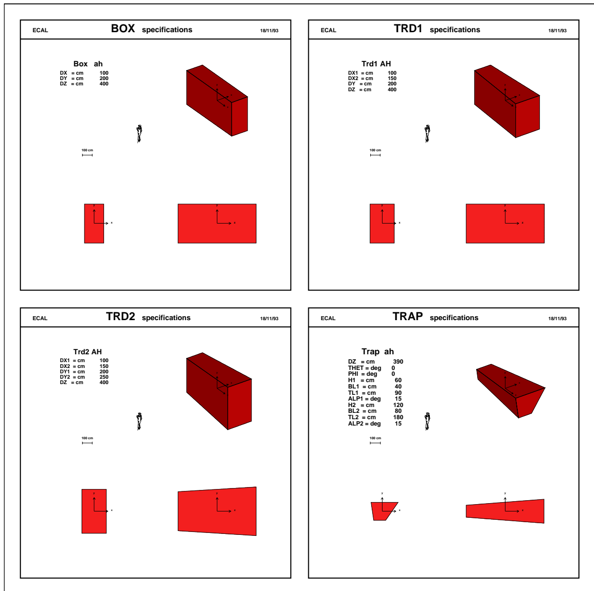
Figure 21: shapes BOX, TRD1, TRD2, TRAP
