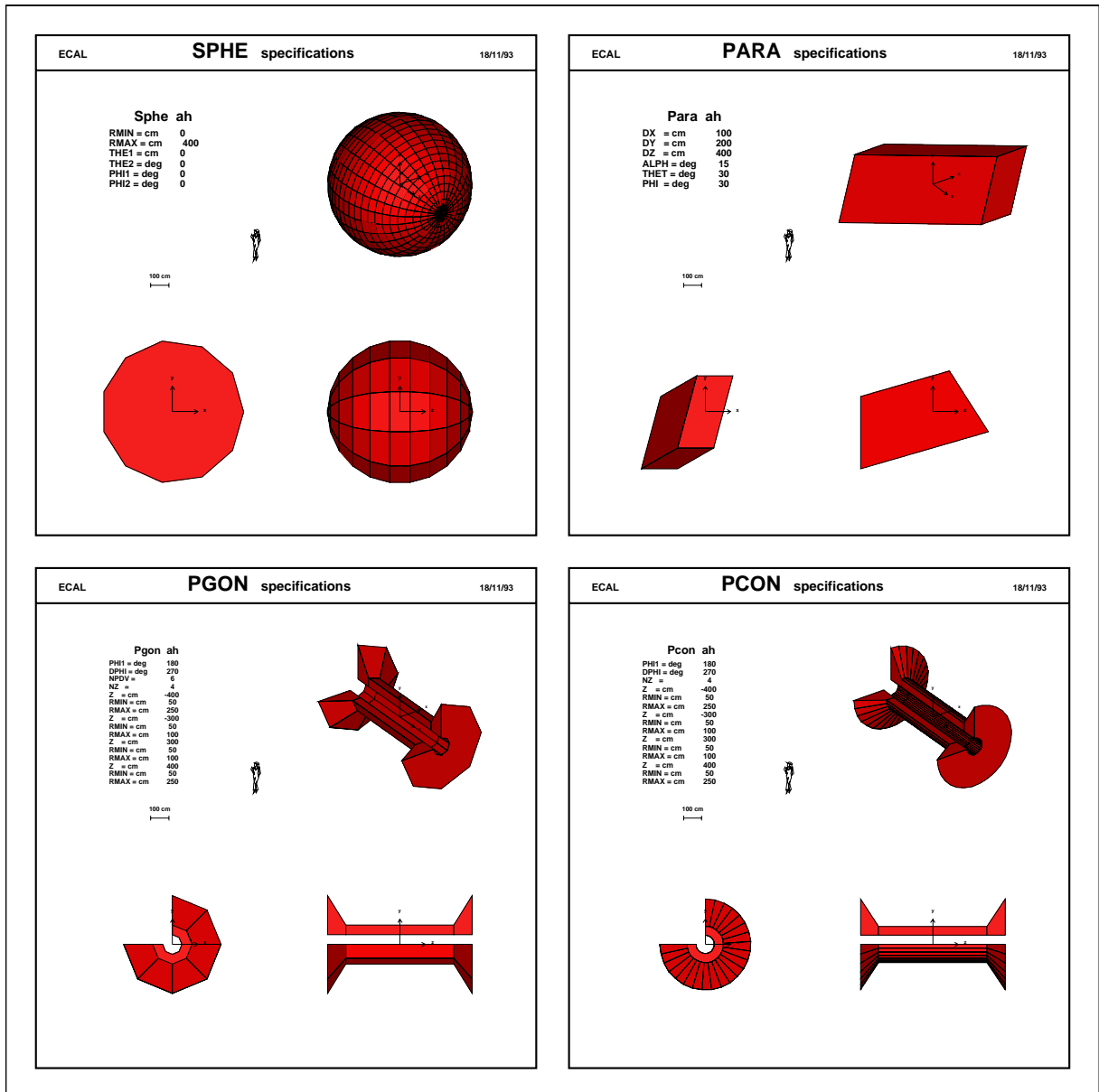
Figure 23: shapes PARA, SPHE, PGON, PCON
