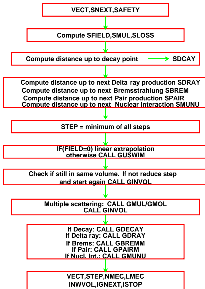
Figure 57: GTMUON block diagram
