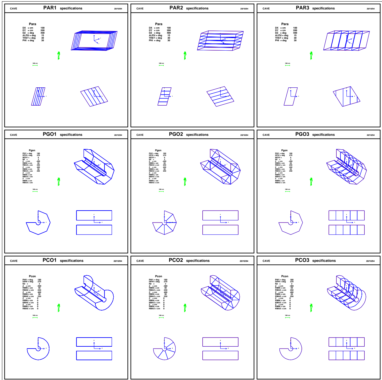
Figure 28: shapes PARA, PGON, PCON
