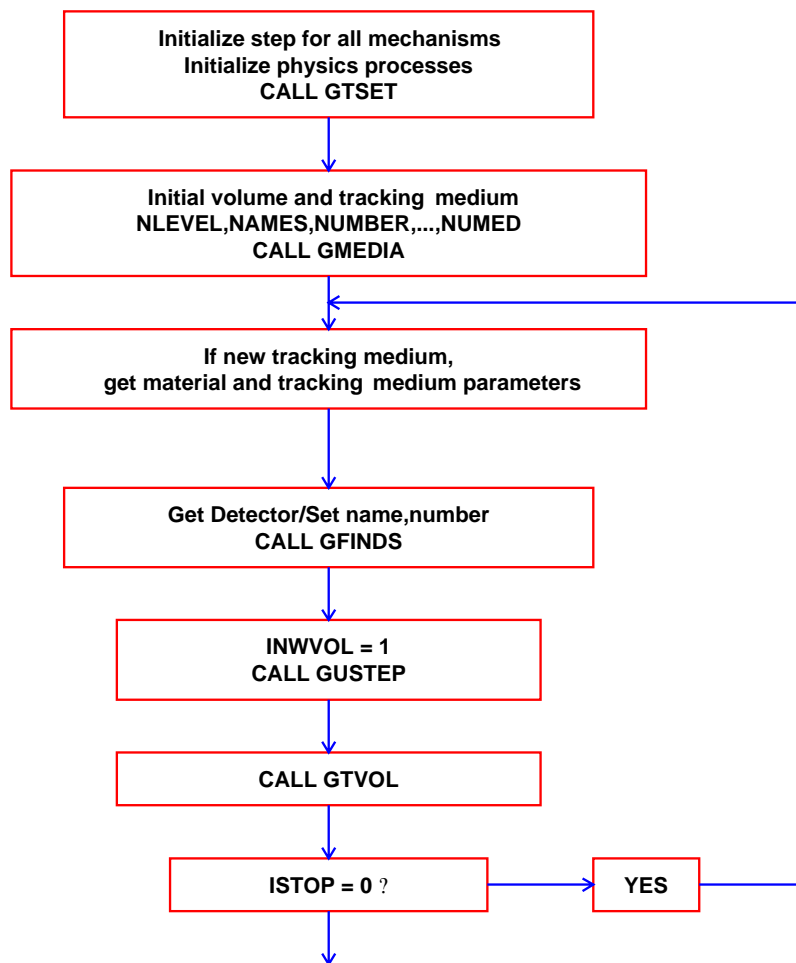
Figure 50: GTRACK block diagram
