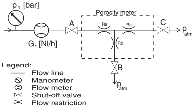
FIG. 12. Equivalent lumped system of test setup.
