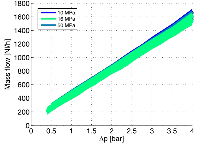
FIG. 14. (Color) Radial flow in cables with enhanced insulation. Vertical compression of 10, 16, and 50 MPa.
