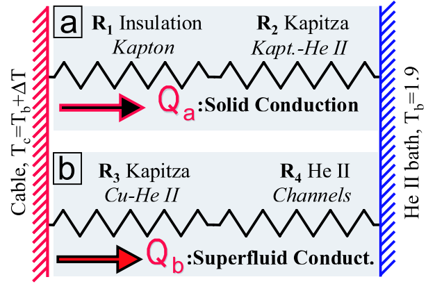
FIG. 2. (Color) Schematization of heat transfer path through porous insulation.
