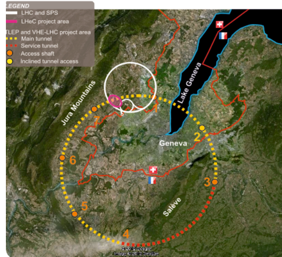
Figure 2: Map of existing CERN tunnels, the preferred option for the 80km tunnel and the linac-ring LHeC project area. The ring-ring LHeC is not highlighted.
