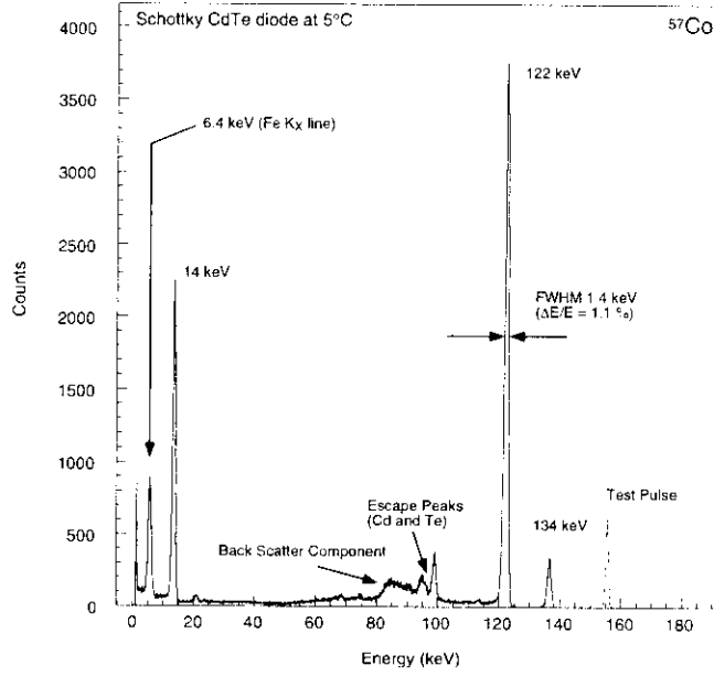
Fig. 3. ^{57}\text{Co} spectrum obtained with the 2\text{ mm} \times 2\text{ mm} Schottky CdTe detector of thickness 0.5 mm. It was operated at 5^\circ\text{C} and a bias voltage of 800 V was applied. The time constant of a shaping amplifier was set at 1\ \mu\text{s} .
