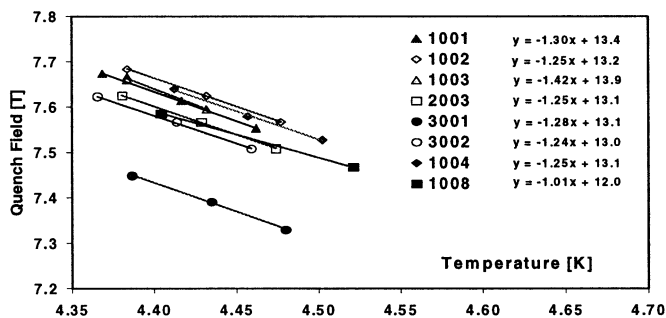
Fig. 2. Quench performance in vicinity of 4.4 K.
