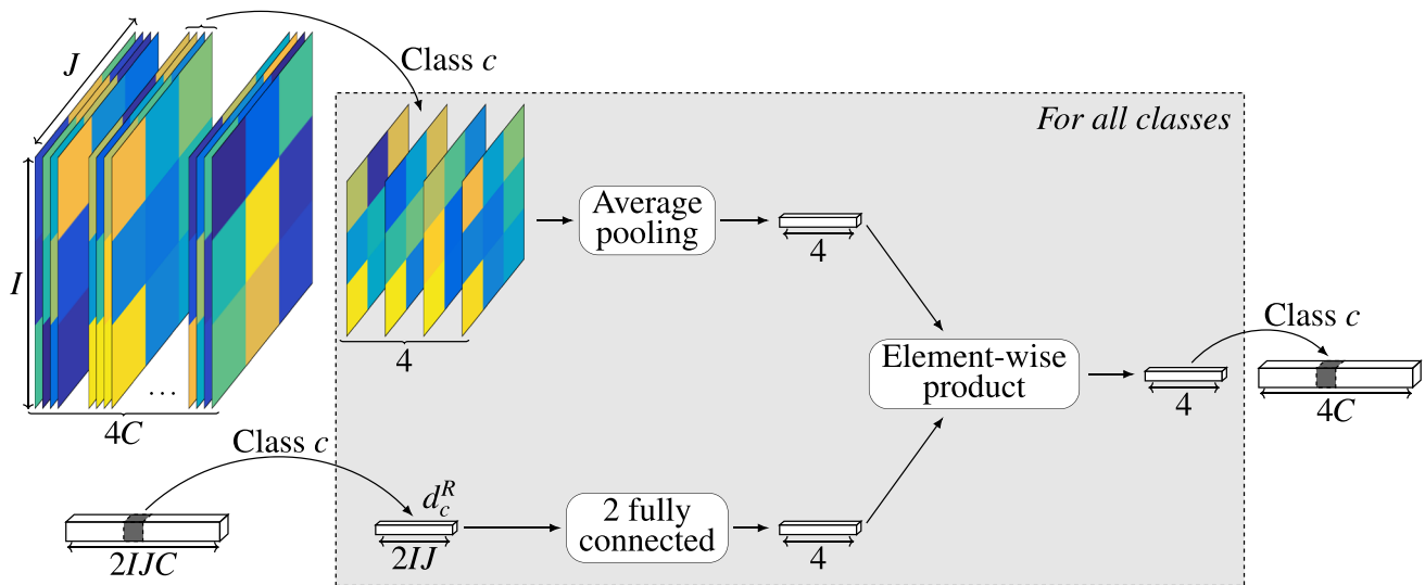
Fig. 5 Deformation-aware global localization refinement. Relocalizations of bounding boxes obtained by averaging pooled values from localization maps (upper path) do not benefit from deformable parts. To do so, displacements of parts are forwarded through two fully connected
