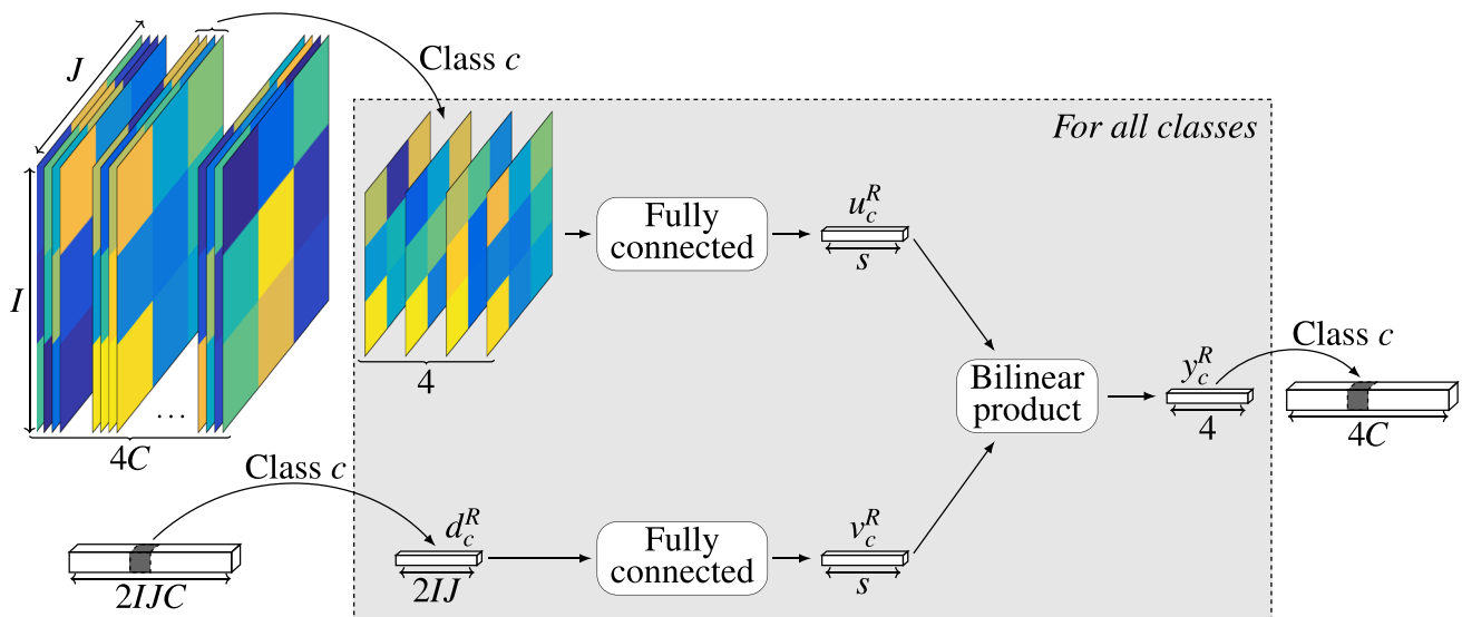
Fig. 6 Deformation-aware bilinear localization refinement. For each region and class, both predictions and displacements from all parts are separately embedded into lower dimensional features before feeding a bilinear product layer (i.e. a Tucker decomposition) to yield final local-
