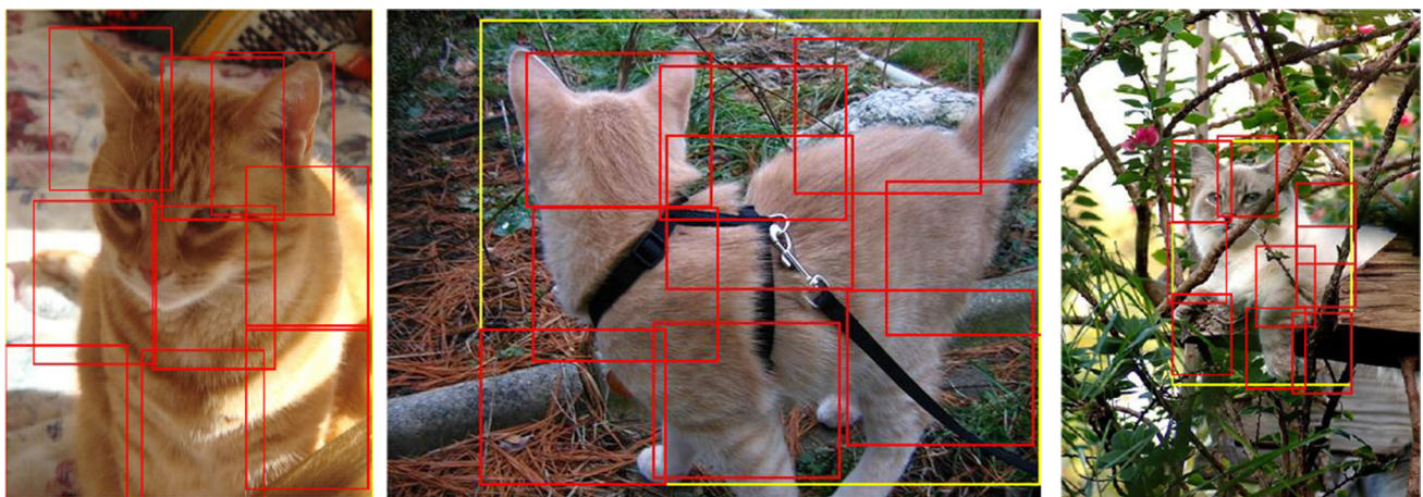
Fig. 9 Examples of deformations of parts from DP-FCN. Initial region proposals are shown in yellow and deformed parts in red. Only 3 \times 3 parts are displayed for clarity (Color figure online)
