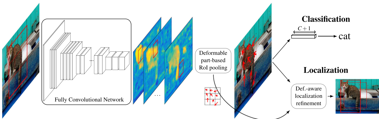
Fig. 2 Architecture of DP-FCN. It is composed of a FCN to extract dense feature maps with high spatial resolution (Sect. 3.1), a deformable part-based RoI pooling layer to compute a representation aligning parts (Sect. 3.2) and two sibling classification and localization prediction
