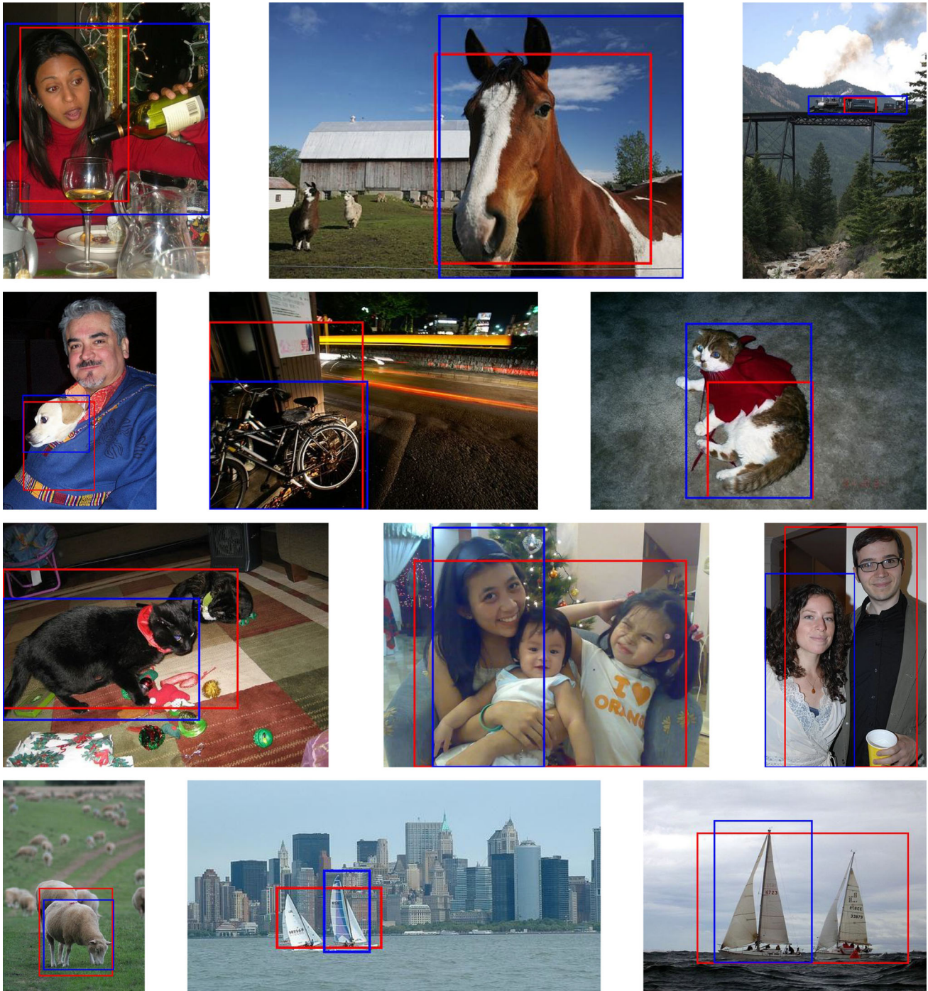
Fig. 7 Comparison of detections from R-FCN (red) and DP-FCN (blue). DP-FCN tightly fits objects (first two rows) and separates close instances (last two rows) better than R-FCN (Color figure online)
