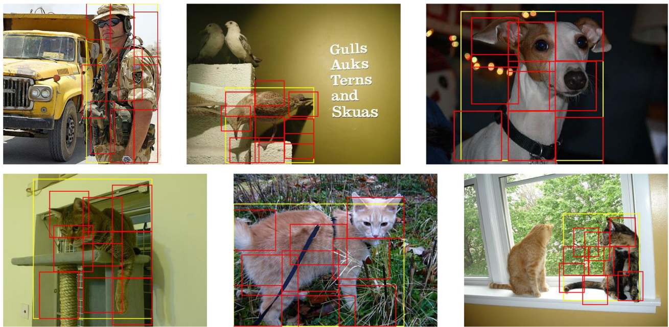
Fig. 10 Examples of deformations of parts from DP-FCN2.0. Initial region proposals are shown in yellow and deformed parts in red. Only 3 \times 3 parts are displayed for clarity (Color figure online)
