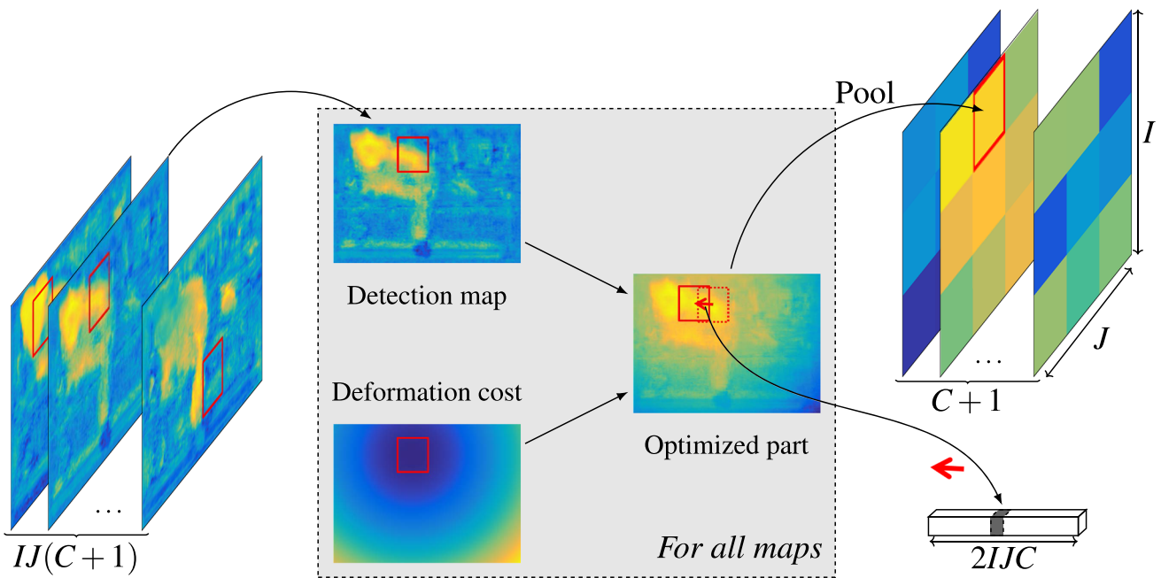
Fig. 3 Deformable part-based RoI pooling with independent deformations. Each input feature map corresponds to a part of a class (or background). Positions of parts are optimized separately within detection maps with deformation costs as regularization, and values are
