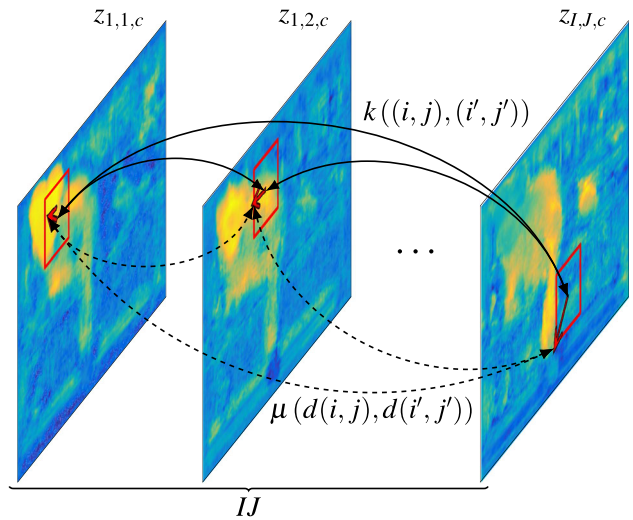
Fig. 4 Visualization of pairwise potentials of CRF between parts for a region of a class c . Interactions between all IJ parts are taken into account through pairwise potentials \phi_p . These are composed of two main terms: a kernel k controlling the strength of the interactions according to the distances between parts, and a compatibility function \mu encouraging similarity of displacements
