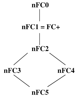
Fig. 2. The hierarchy of the algorithms with respect to the number of visited nodes. Two algorithms are connected by an edge if the set of nodes visited by the lower is a subset of the set of nodes visited by the upper.
