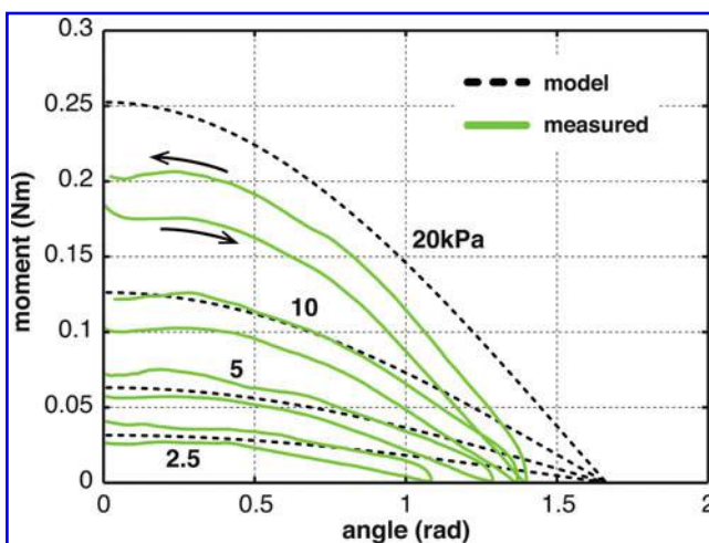
FIG. 7. The moment-angle relationship of the angular pouch motor with hinged structure at various pressure. Solid lines show measured data, and dotted lines show the corresponding theoretical curves. The arrows indicate outward and return of the hysteresis curve. Color images available online at www.liebertpub.com/soro
