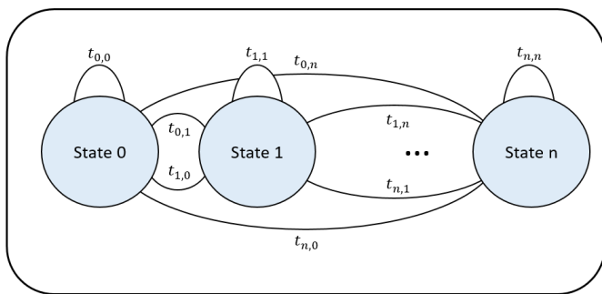
Fig. 10. An example of a Discrete-time Markov Chain, in which states are represented by circles, and transition probabilities between states are assigned by t_{a,b} .
