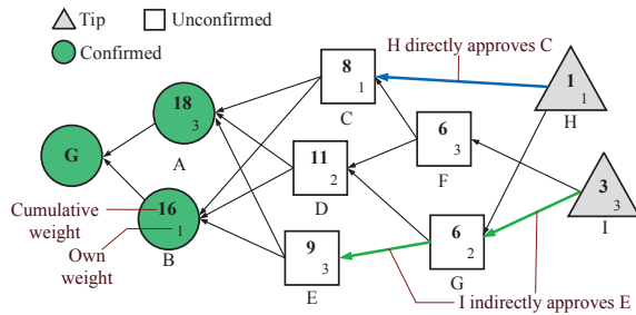
Fig. 2: An example of Tangle
