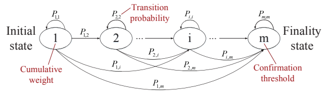
Fig. 4: Markov chain model for the consensus process of a new transaction
