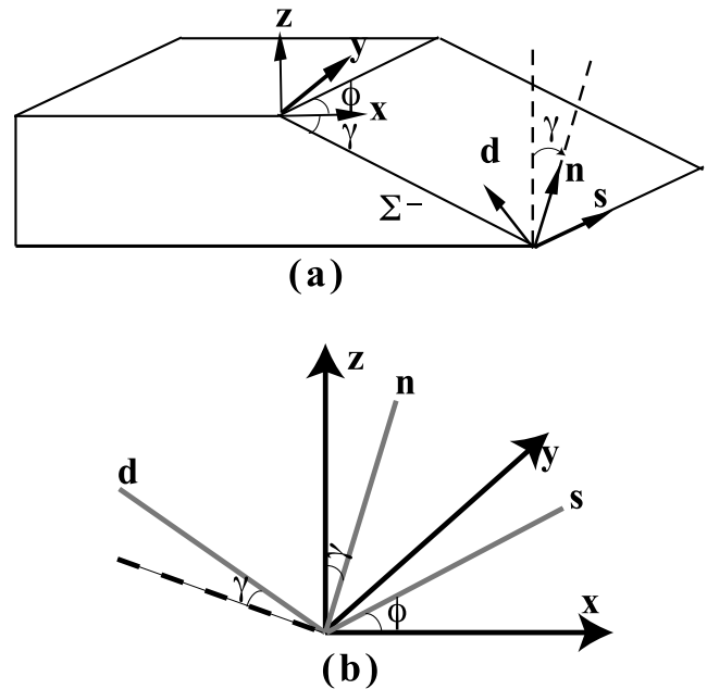
Figure A1. (a) \Sigma^- side of the fault plane, taken as the footwall for the dipping fault, and chosen arbitrarily if the fault is vertical. \phi is the angle measured from the x axis to the surface trace of the fault corresponding with strike direction \vec{s} , counterclockwise about z . \gamma is the angle from the x - y plane, at the right of the strike direction, to the fault plane. s , d and n are the strike, updip, and outward normal vectors, respectively, to the \Sigma^- surface. (b) Various angles between the (s, d, n) and (x, y, z) coordinate systems.
