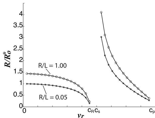
Figure 15. Variation in the scaled size of the process zone R/R_0^* with rupture velocity v_r . R_0^* is the size of the process zone at static limit for a semi-infinite shear crack. c_R , c_s , and c_p are the Rayleigh and S - and P -wave speeds of the medium, respectively.
