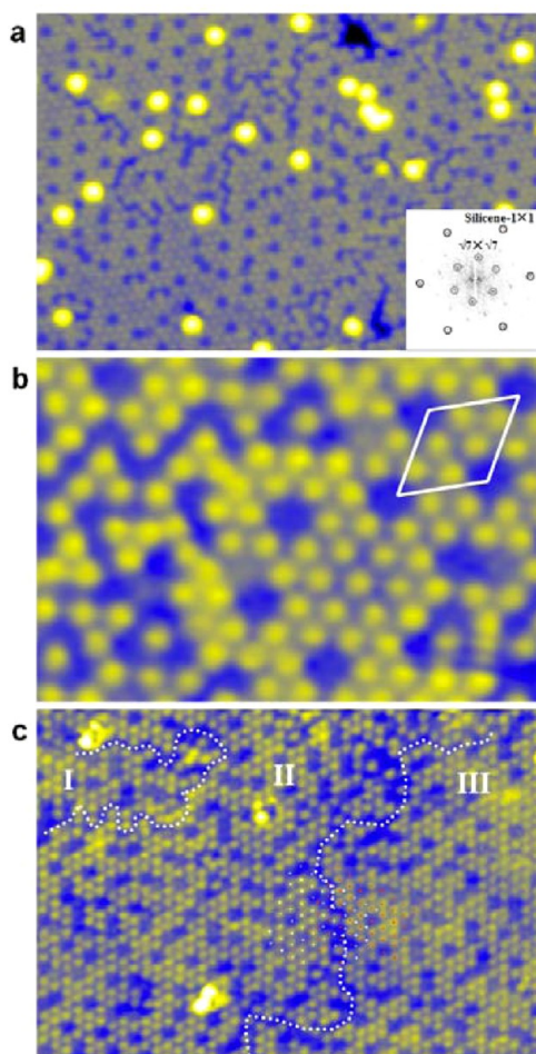
Figure 2. Full hydrogenation of the silicene (2\sqrt{3}\times 2\sqrt{3})R30^\circ phase on Ag(111). (a) STM image ( 17\times 12 nm 2 , V_{\text{tip}} = 0.50 V, I_{\text{set-point}} = 430.0 pA) of the fully hydrogenated silicene (2\sqrt{3}\times 2\sqrt{3})R30^\circ phase. The inset is the result of FFT of (a), showing six spots corresponding to silicene- 1\times 1 lattice. (b) High-resolution STM image ( 5\times 4 nm 2 , V_{\text{tip}} = 0.20 V, I_{\text{set-point}} = 281.0 pA) of the hydrogenated (2\sqrt{3}\times 2\sqrt{3})R30^\circ phase. The white rhombus marks the periodically ordered hole sites with \sqrt{7}\times\sqrt{7} structure with respect to the silicene 1\times 1 lattice, which agrees well with the \sqrt{7}\times\sqrt{7} spots observed in the inset of (a). (c) STM image ( 15\times 10 nm 2 , V_{\text{tip}} = 0.43 V, I_{\text{set-point}} = 80.0 pA) of the hydrogenated silicene (2\sqrt{3}\times 2\sqrt{3})R30^\circ phase shows three domains (marked by I, II, and III). The domain boundaries are labeled by white dotted lines. The small white and red dots correspond to the lattice of the bright spots in II and III domains, respectively. One lattice is exactly located in the hollow site of the other lattice.
