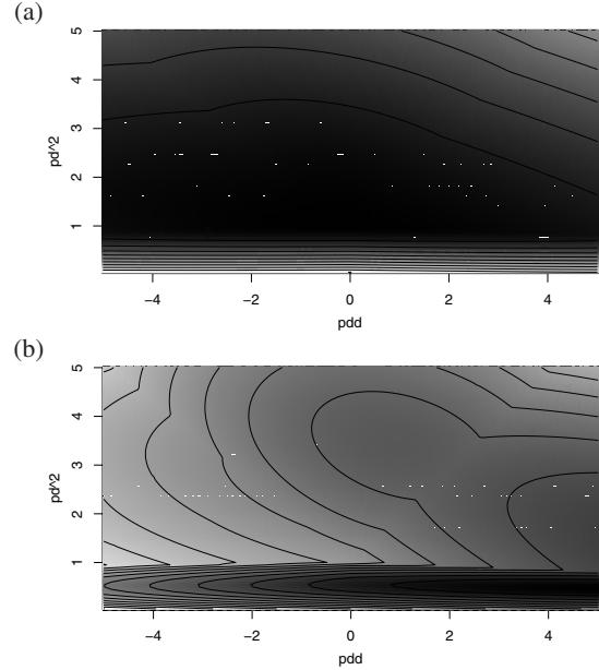
Figure 7: Zoomed-in versions of the near normal speed regions of (a) the force matching and (b) the force minimization examples shown in 6. Notice that force minimization has many more minima than force matching.
