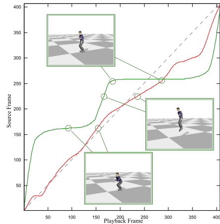
Figure 9: Two retimings of 16_03 [CMU]. In red, lower gravity produces a longer flight time and slower takeoff. In green, higher gravity produces a shorter flight time and faster takeoff. (The plateaus in the high-gravity timing are due to the length being constrained.)
