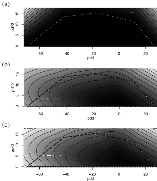
Figure 6: Objective function component magnitude in the \dot{p} \times \dot{p}^2 plane, evaluated at frame 143 of the 16_06 jump from [CMU]. The feasible region is superimposed. (a) is the feasible region distance. (b) is force matching to regular speed. (c) is force minimization.
