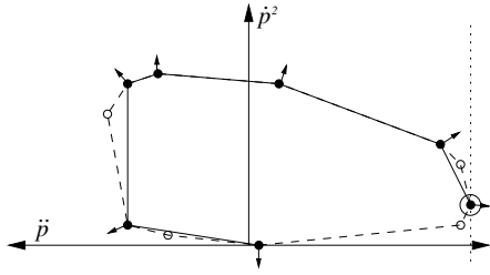
Figure 4: The process of finding a hull in the (\dot{p}, \dot{p}^2) plane. The direction of maximization has been swept counterclockwise from straight down to right. The arrow at each point indicates the direction it was found at. The solid lines are the hull found so far, with the circled vertex the most recently added (the dotted line is perpendicular to the direction of maximization; notice no other vertex crosses it). The dashed lines are the true hull. Even though some vertices may be missed, the found hull will lie inside the true hull.
