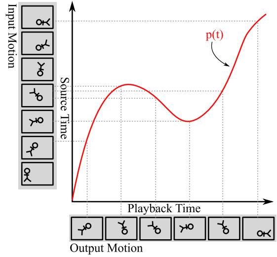
Figure 2: The result of our retiming will be a cubic spline, p(t) , which will map from output time to input time. The output frame at time t is the input frame from time p(t) .
