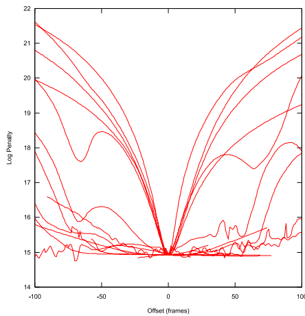
Figure 13: The change in the penalty with respect to the offset of each control point from the local minimum penalty position.
