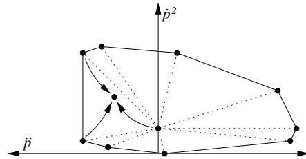
Figure 5: Contact forces for a new point in the plausible region are interpolated from the containing triangle's corners.
