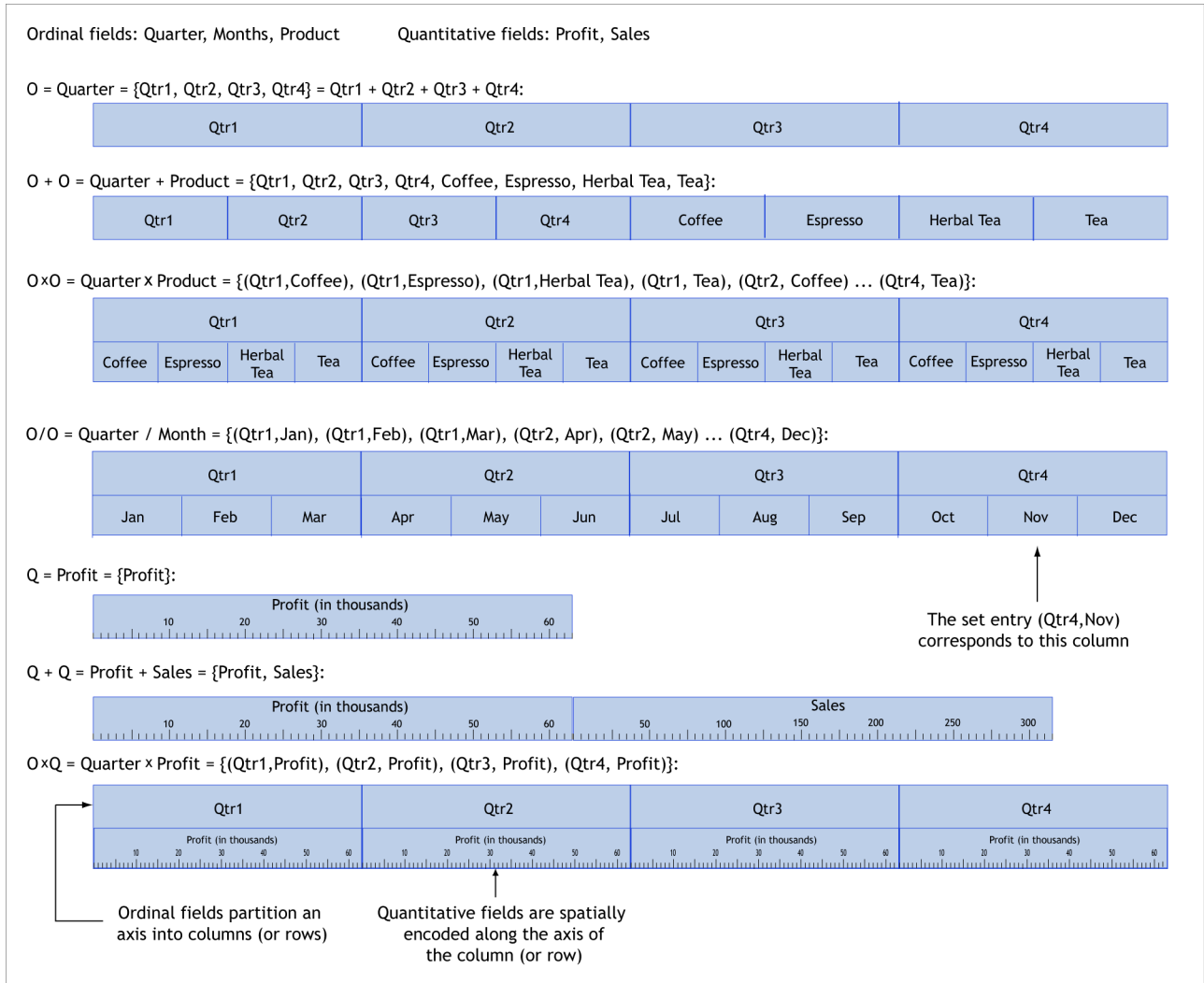
Figure 2: The graphical interpretation of several expressions in the table algebra. Each expression in the table algebra can be reduced to a single set of terms, and that set can then be directly mapped into a configuration for an axis of the table.
