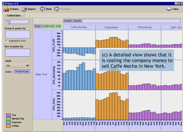
Figure 6: An example scenario demonstrating the capabilities of Polaris for exploratory analysis of multi-dimensional databases. The data displayed is for a hypothetical coffee store chain, and the analyst is searching for ways to reduce the company's expenses.
