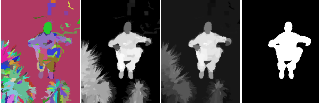
Figure 5. Image regions generated by Felzenszwalb and Huttenlocher’s segmentation method [9] (left), region contrast based segmentation with (left-middle) and without (right-middle) distance weighting. Incorporating the spatial context, we get a high quality saliency cut (right) comparable to human labeled ground truth.
