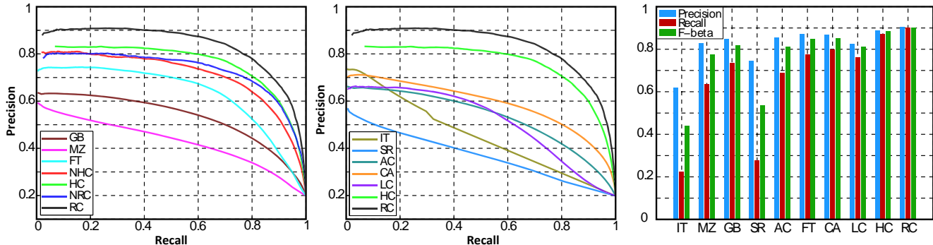
Figure 7. Precision-recall curve for naive thresholding of saliency maps using 1000 publicly available benchmark images. (Left, middle) Different options of our method compared with GB[12], MZ[19], FT[2], IT[15], SR[13], AC[1], CA[10], and LC[29]. NHC denotes naive version of our HC method with color space smoothing disabled, and NRC denotes our RC method with spatial related weighting disabled. (Right) Precision-recall bars for our saliency cut algorithm using different saliency maps as initialization. Our method RC shows high precision, recall, and F_\beta values over the 1000 image database. (Please refer to project webpage for respective result images.)
