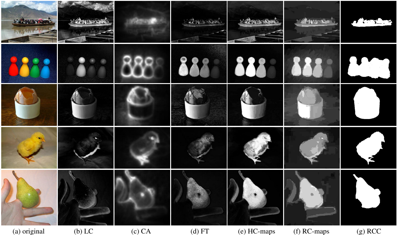
Figure 6. Visual comparison of saliency maps. (a) original images, saliency maps produced using (b) Zhai and Shah [29], (c) Goferman et al. [10], (d) Achanta et al. [2], (e) our HC and (f) RC methods, and (g) RC-based saliency cut results. Our methods generate uniformly highlighted salient regions (see project webpage for all results on the full benchmark dataset).
