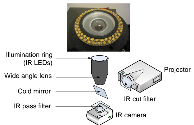
Figure 7. Schematic drawing of our omni-directional projector-camera unit. The detail image shows the wide-angle lens and the IR illumination ring.
