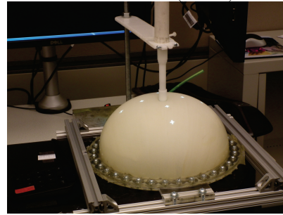
Figure 4: The device used to measure precision for deformation distance and position of our prototypes. Note: the device was angled to test different inclinations on the hemisphere to move along the surface normal.
