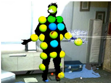
Figure 3. A Unity view showing sphere collider proxies used to determine run-time collisions between game objects (e.g., the incoming fireball) and dynamic surface geometry (e.g., users).
