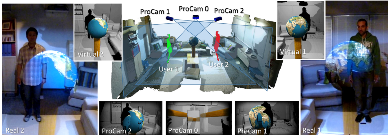
Figure 1. Dyadic projected spatial augmented reality enables two users to interact with a shared virtual scene and each other in a face to face arrangement. Center: Room geometry, user geometry and projector camera pairs are illustrated. Virtual 1 & 2: The desired view for each user is rendered offscreen. ProCam 0, 1 & 2: Projected graphics are warped to account for surface geometry, including the other user. Real 1 & 2: Each user's resulting view compares well with the desired view (Virtual 1 & 2).
