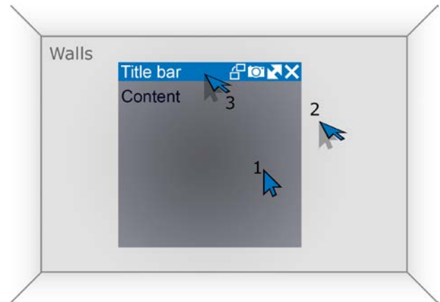
Figure 4. Cursors in MeetAlive. (1) Desktop Cursor is a virtual copy of the standard OS cursor and it shows that the participant is working within their own desktop. The cursor is flat. (2) Room Cursor is activated when the participant moves the cursor out of their own desktop. It is rendered lifted. (3) The participant can access room-related functionalities and arrange content in the room with the room cursor and the title bar icons.
