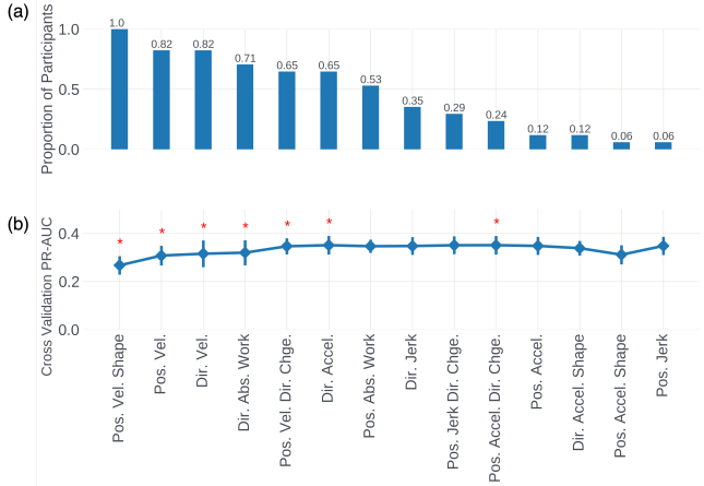
Figure 3: Results of the RFA. (a) The proportion of participants that retained a given feature. (b) Features that were retained from the RFA within participants were iteratively added, from the most retained to the least retained. Each point depicts the average PR-AUC from the 5-fold cross-validation. The error bars depict 95% confidence intervals. Asterisks correspond with features that increased the PR-AUC relative to the previous benchmark and were used in follow-up model evaluations.
