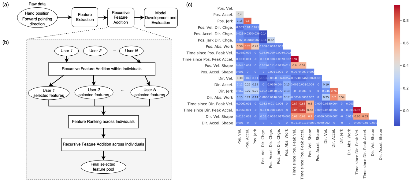
Figure 2: Feature-based logistic regression model development. (a) The feature exploration pipeline. Hand features were first extracted from the raw hand motion time series data. To identify a set of predictive features, training samples were generated using a sliding window approach followed by an RFA method. A logistic regression model leveraged this set of selected features. (b) A flowchart of the RFA method. (c) The feature correlation matrix.
