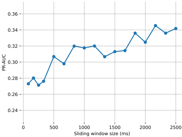
Figure 4: The effect of sliding window size on the Logistic Regression-based RIDS model.
