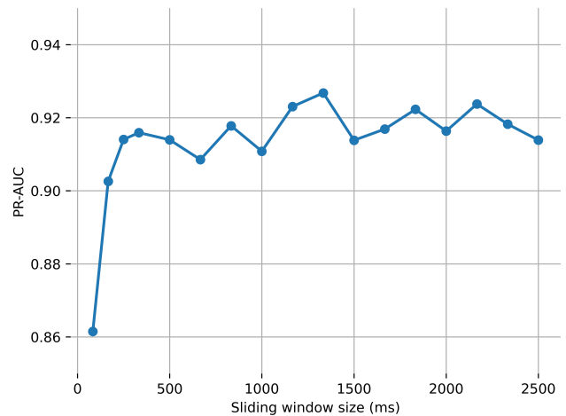
Figure 6: The effect of the sliding window size on the TCN model.
