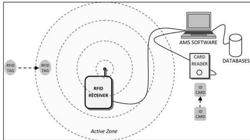
Figure 5: The implementation architecture of the system.
