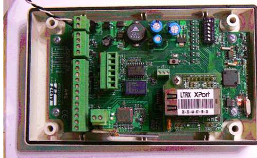
Figure 2: LX 2002 Radio Receiver for Dual Frequency Tag.
