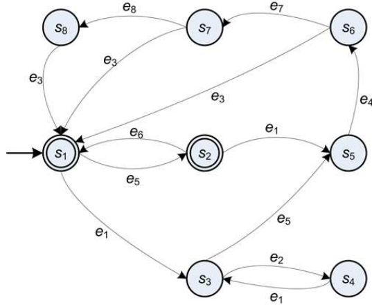
Figure 3: The diagram of the finite state machine.
