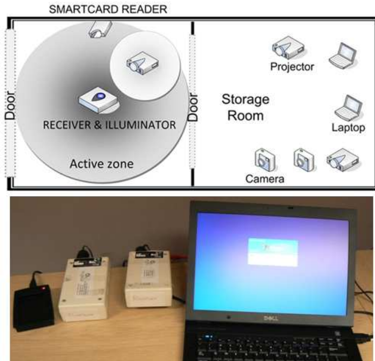
Figure 13: Deployment of the system: Receiver, Illuminator, Card Reader, and Store, and the devices next to the laptop.
