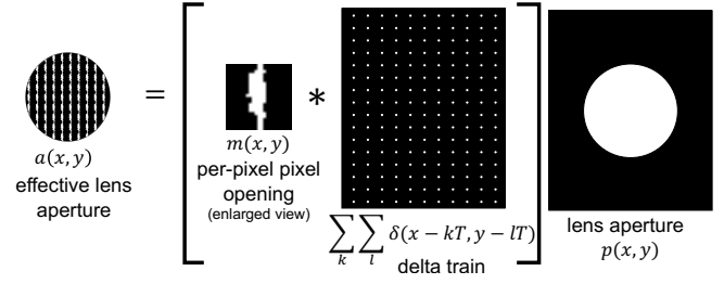
Fig. 3. Modeling the effective aperture of an under-panel camera
