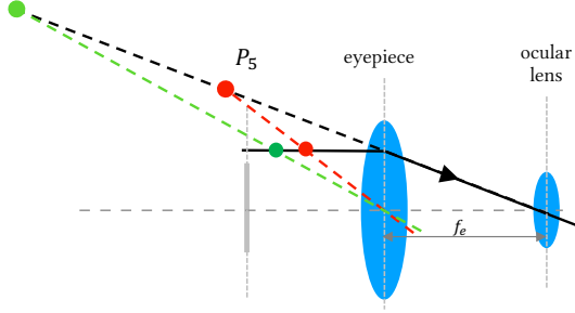
Fig. 4. Position of the eye. We require that the eye be placed at the focal plane of the eyepiece, i.e., a distance of f_e from the eyepiece. This placement is important as it ensures that an axially translating point on the display remains at the same viewing angle at the eye.
