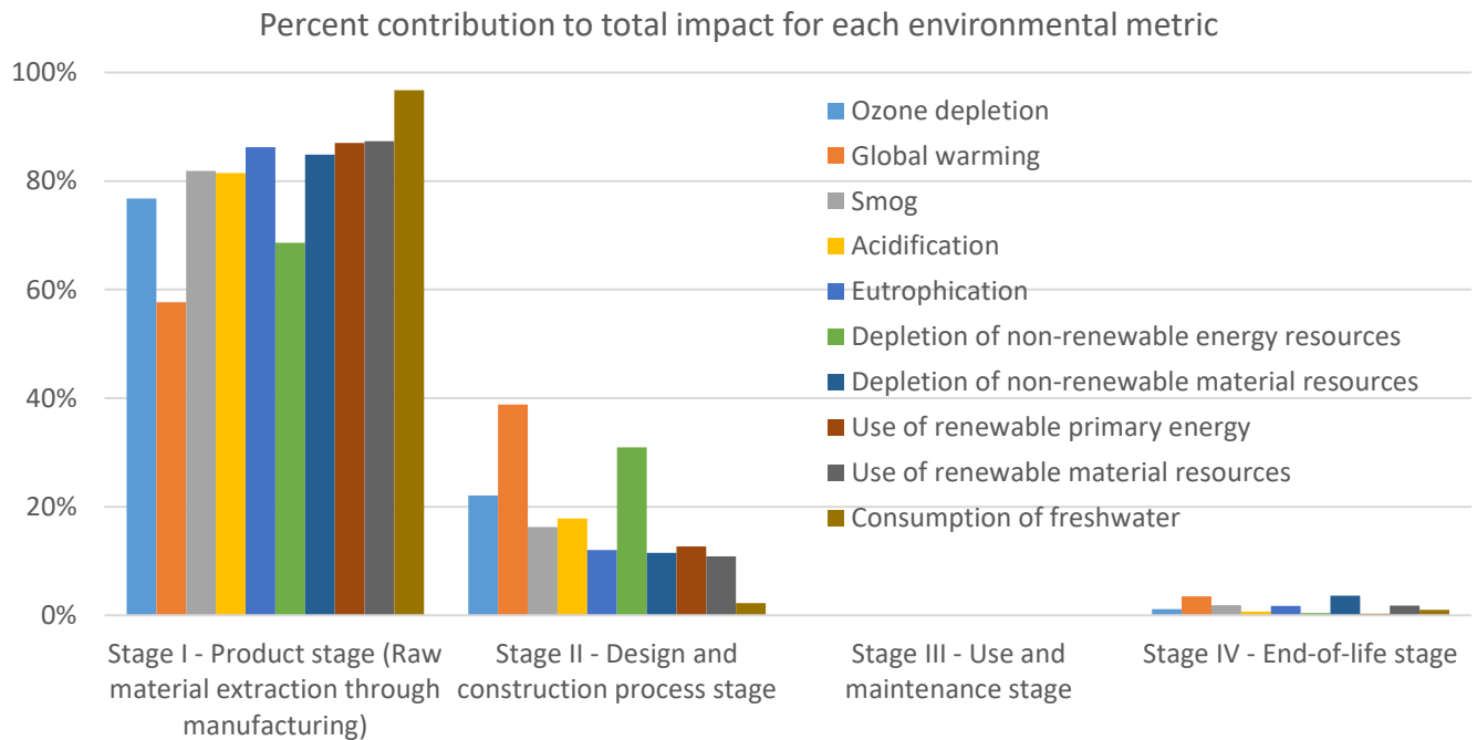
Figure 3 - Graphical impacts for the average SPEEDHIDE ® Pro EV Zero product showing % contribution by life cycle stage. Results for individual products are not expected to differ substantially from the results shown above
