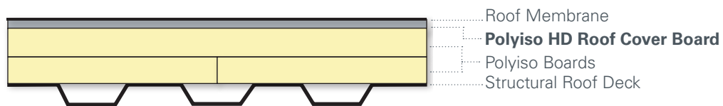
Figure 1. Typical Roof Assembly with Polyiso HD Roof Cover Board Installed Between the Insulation and the Roof Membrane.
