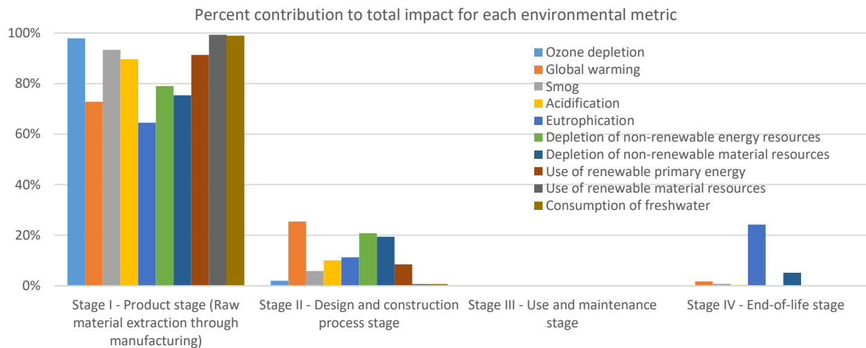
Figure 3 - Graphical impacts for the average PITT-GLAZE WB1 Water-Borne Acrylic Epoxy product showing % contribution by life cycle stage
