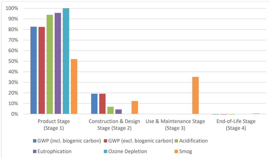
Figure 2. Impact Category Result Breakdown by ISO 21930 Stage for Average DuraCraft™ Acrylic Exterior Latex Formulation.
