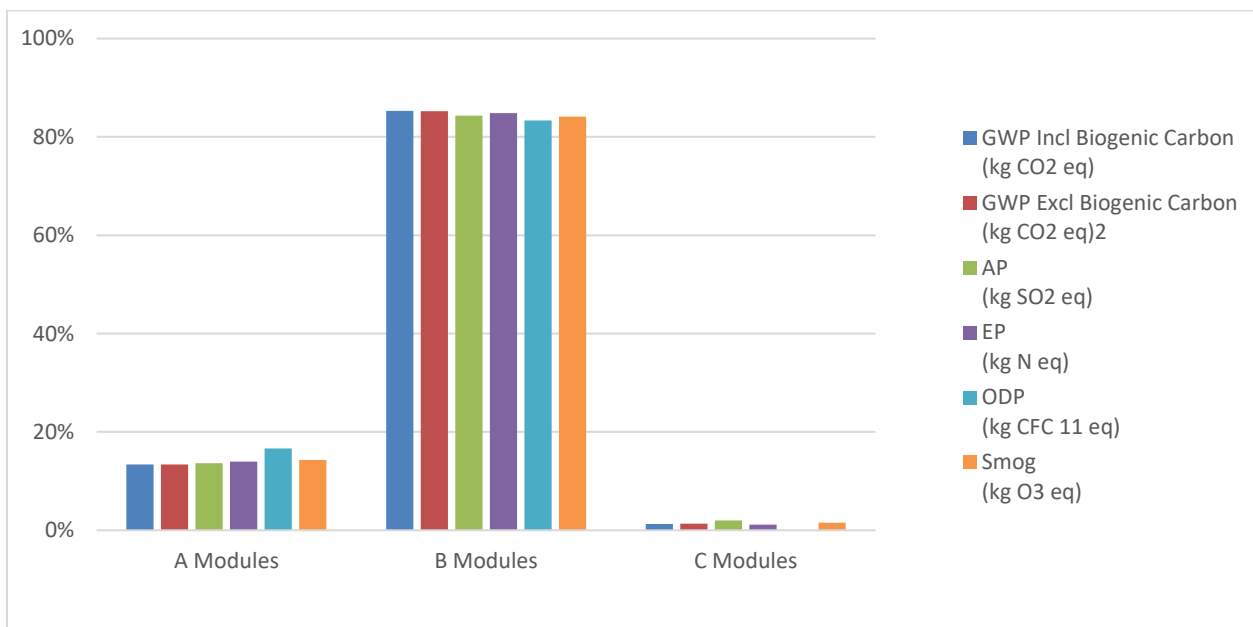
Figure 3. Averaged Floor Coating LCIA Impact Distribution by ISO 21930 Modules
