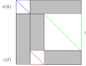
Figure 3: Illustration of the decomposition of a permutation in S_n(123, 231) .
