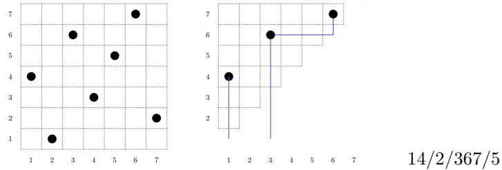
Figure 1: Graphical representation of \sigma = 4\ 1\ 6\ 3\ 5\ 7\ 2 with its excedance board and its associated partition.
