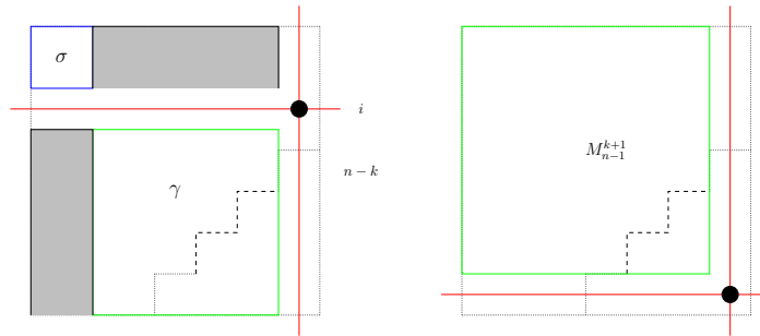
Figure 2: Illustration of the two cases studied in the proof of Theorem 4.
