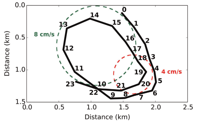
Fig. 10. Position-time plot of a track of a single iceberg shown in Fig. 9. The data are shown at hourly intervals. Hour 0 is August 17, 13:00. The velocities range between 4 and 11 cm/s. Note that the iceberg velocity decreases as it gets closer to the glacier front. The figure also shows theoretical inertial radii, which are calculated for a speed of 4 cm/s (300 m radius, 600 m diameter, red) and 8 cm/s (600 m radius, 1200 m diameter, green). The similarity of the theoretical calculations to the measured iceberg path supports the hypothesis that post-outflow currents are dominated by inertial motion. (For interpretation of the references to color in this figure caption, the reader is referred to the web version of this paper.)
