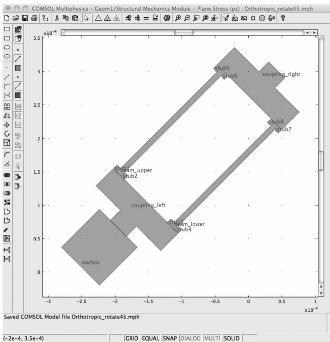
Fig. 6. DETF resonator model drawn in COMSOL, rotated 45^\circ . The structure shown in Fig. 4 was simply rotated 45^\circ counterclockwise.
