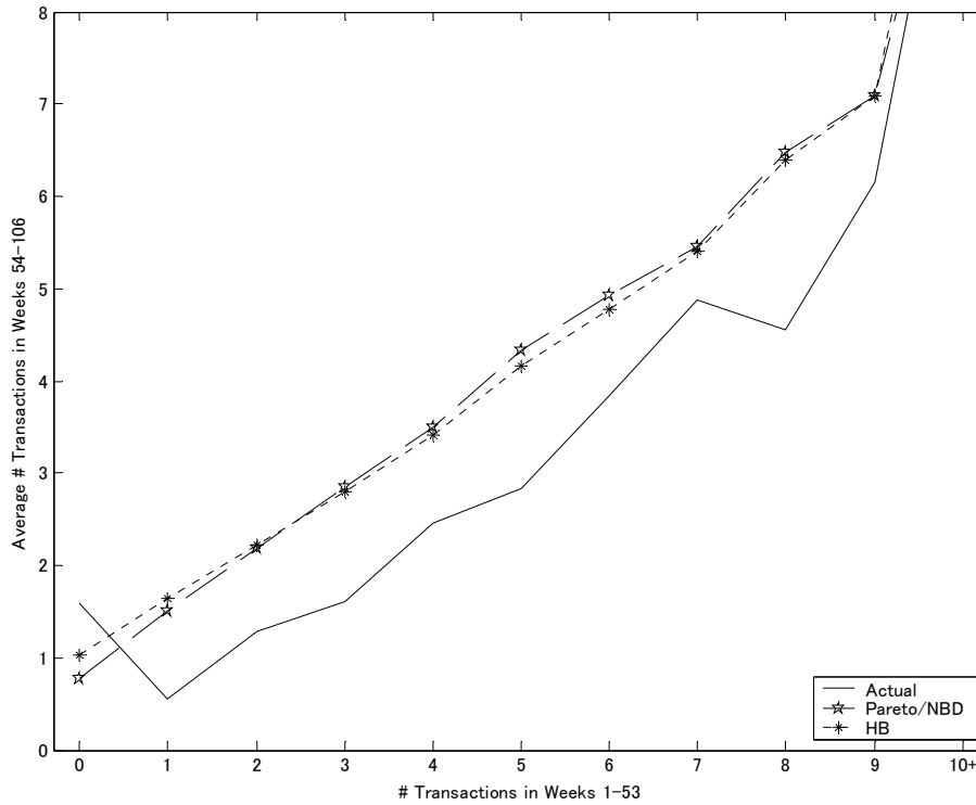
Figure 6. Conditional Expectation of Future Transactions
