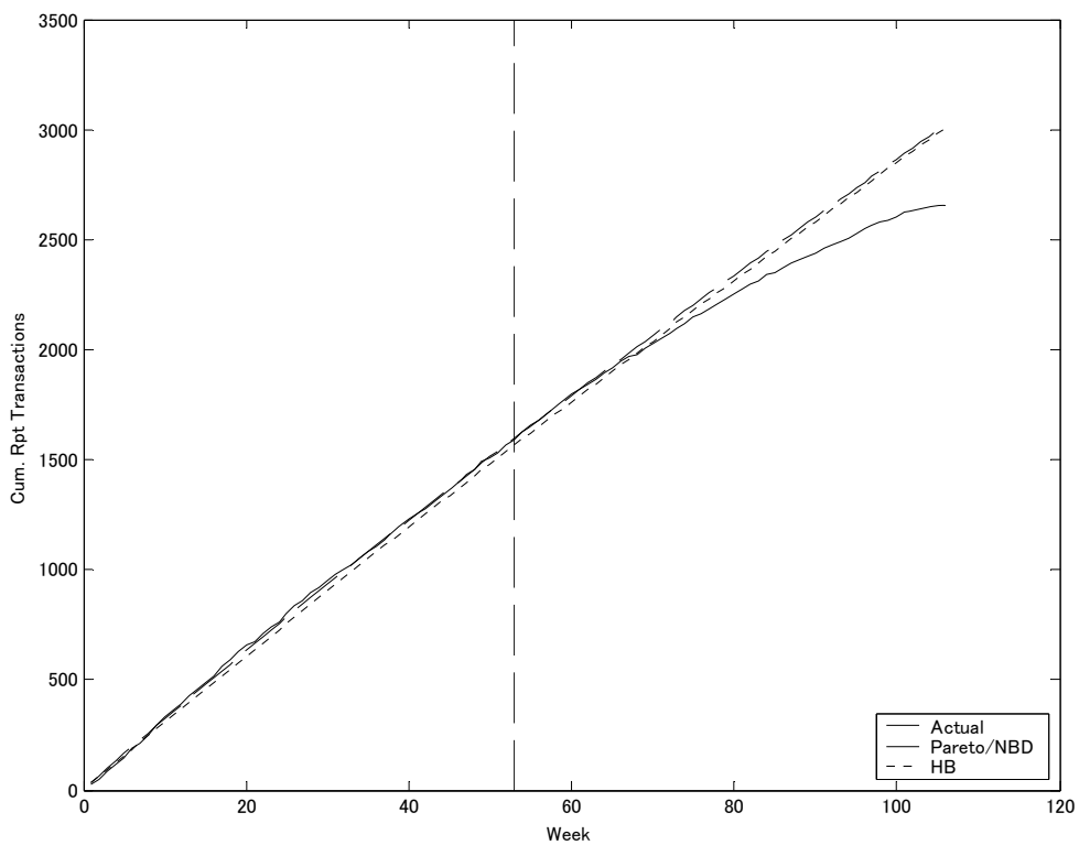
Figure 5. Weekly Time-series Tracking Plot
