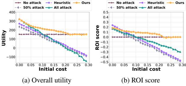
Figure 3: Comparison of attack deployment strategies with increasing attack cost: Decision maker’s behavior model is learned from the data of our human-subject experiment.
