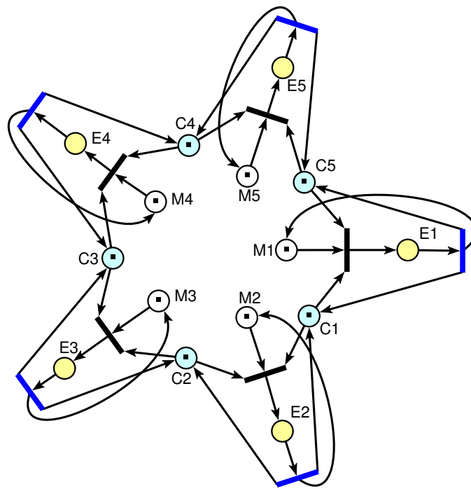
Figure 13: Petri net
