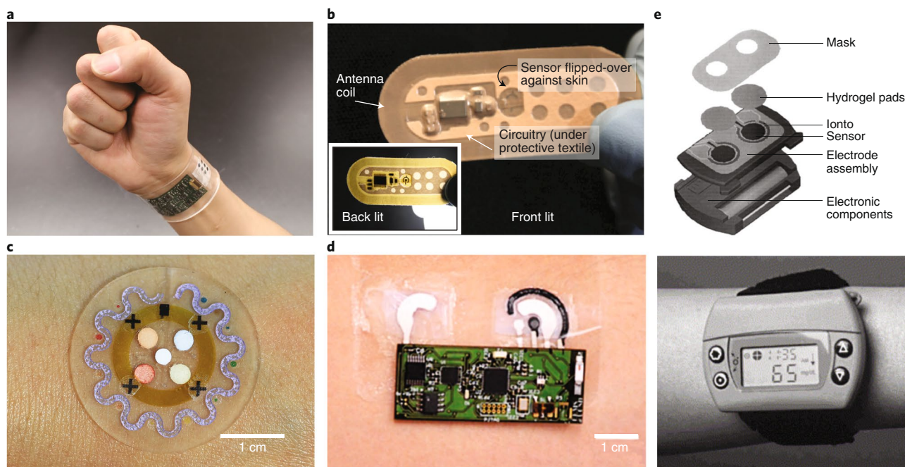
Fig. 3 | Wearable sweat sensors. a , A multiplexed electrochemical system for continuous monitoring of a panel of analytes in sweat, integrated into a ‘smart’ wristband for fitness monitoring. Wireless transmission to a custom phone app allows easy read-out of analyte concentrations. b , A Band-Aid-style patch for continuous detection of ions in sweat, with RFID antenna for wireless signal transmission. c , One-time, colourimetric detection of sweat analytes is realized using colourimetric assay reagents encased in microfluidic wells. d , Screen-printed electrodes on a tattoo substrate achieve ethanol detection in iontophoretic sweat. e , GlucoWatch used reverse iontophoresis for semi-continuous glucose measurement. Credit: reproduced from ref. 6 , Macmillan Publishers Ltd ( a ); ref. 9 , IEEE ( b ); ref. 8 , AAAS ( c ); and adapted from ref. 19 , American Chemical Society ( d ); ref. 37 , AACC ( e , top); ref. 36 , Elsevier ( e , bottom).
