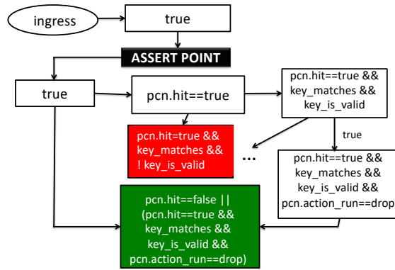
Figure 6: Weakest preconditions.
